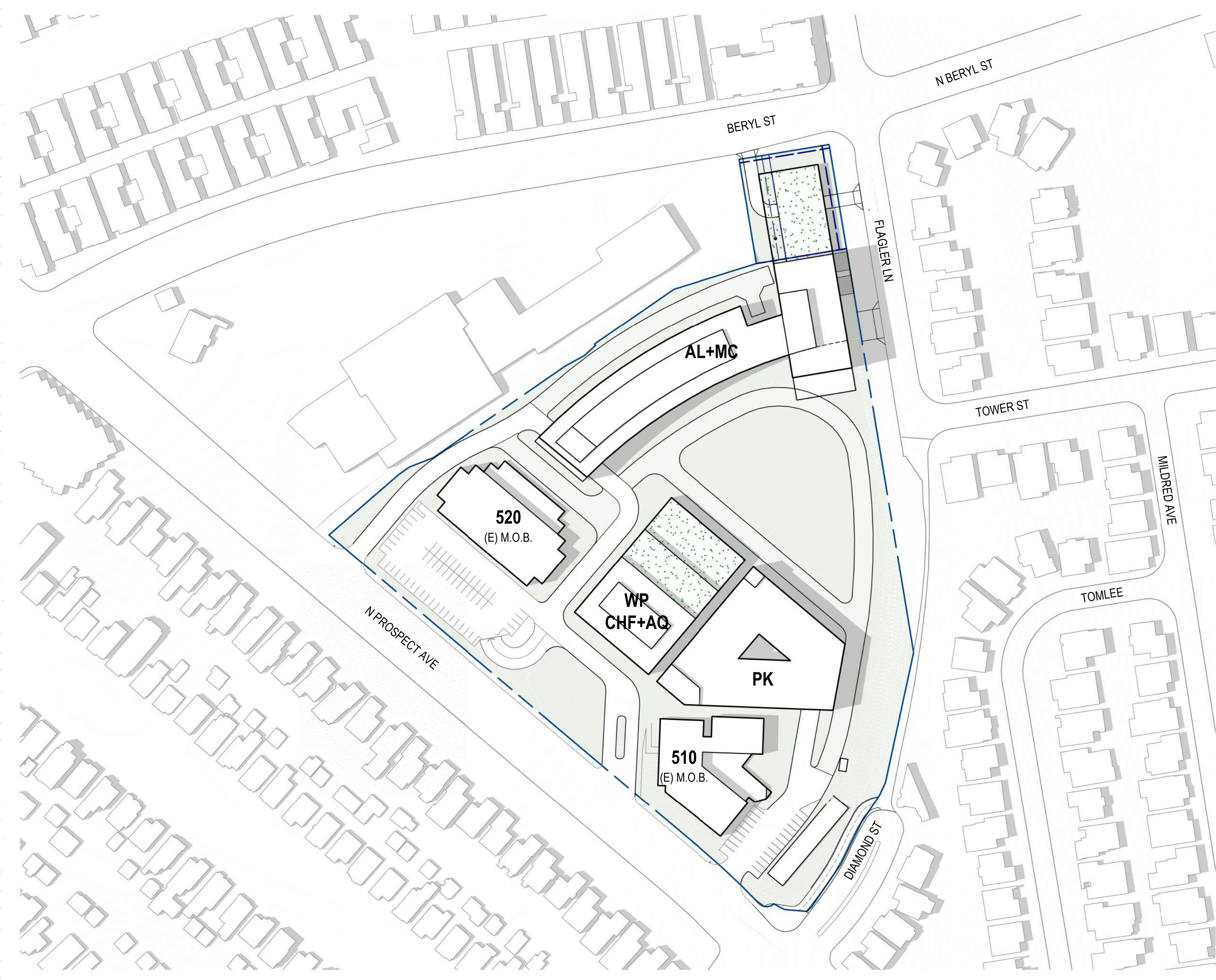
PH2 - SUMMER SOLSTICE 2PM 1" = 100'-0" 4
